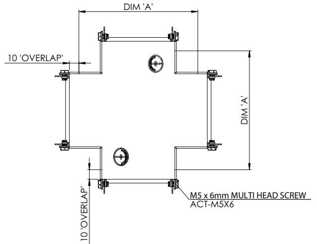
ASB - SCREWBUSH
